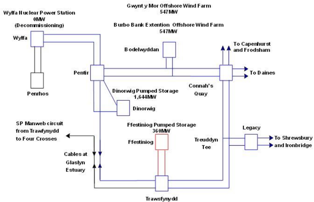
Figure 3.2 – Schematic Diagram of the Transmission System within North Wales
