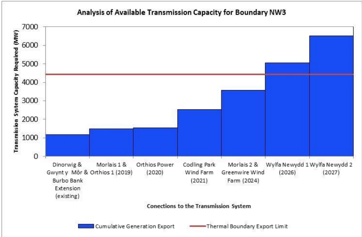
Figure 5.3: NW3 Boundary Export s. Transmission Capacity
