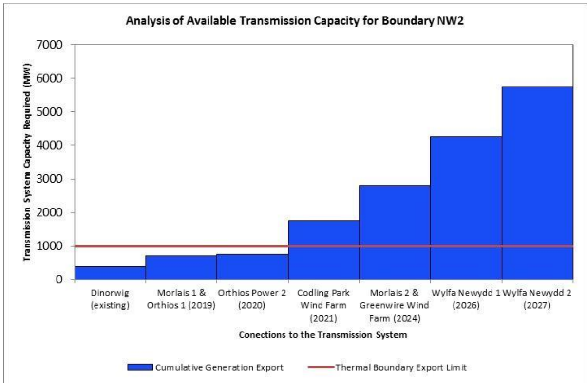
Figure 5.2: NW2 Boundary Export s. Transmission Capacity
