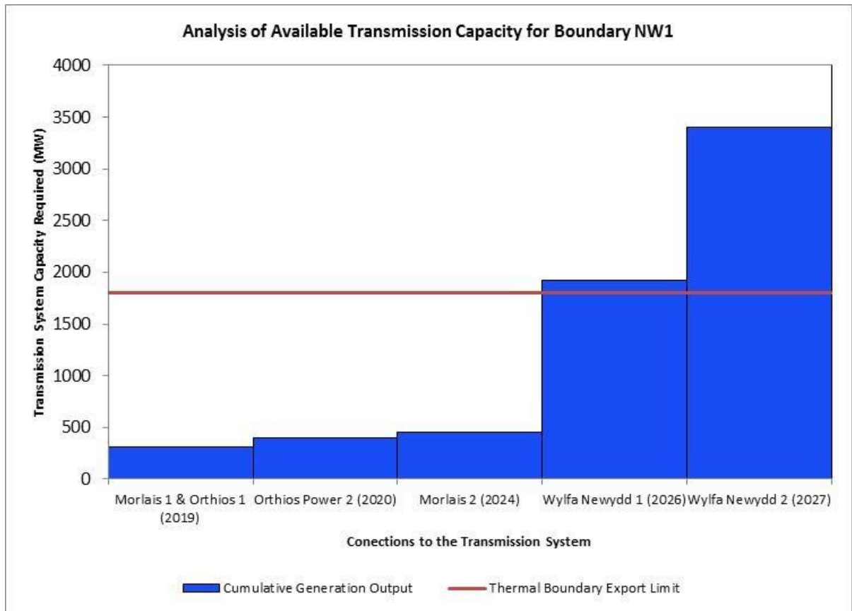
Figure 5.1: NW1 Boundary Exports vs. Transmission Capacity
